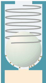
Figure 27: By-pass valve
