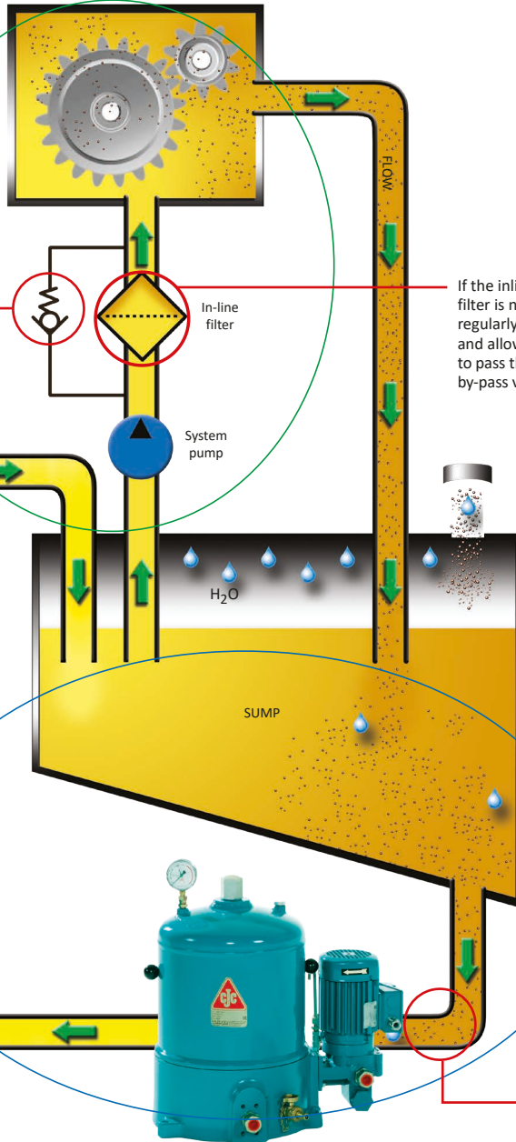
CJC® Offline Oil Filter
