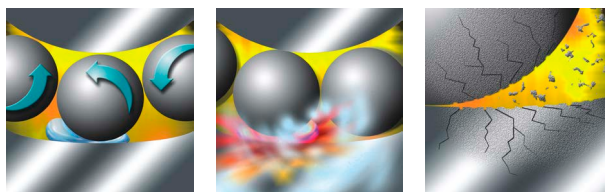
Figure 4: Cavitation and pitting
