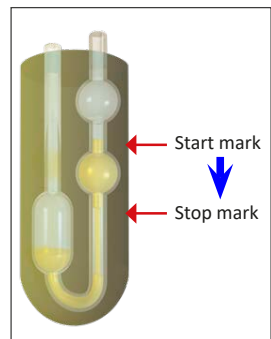
Figure 13: Viscometer measures kinematic viscosity (cSt)
